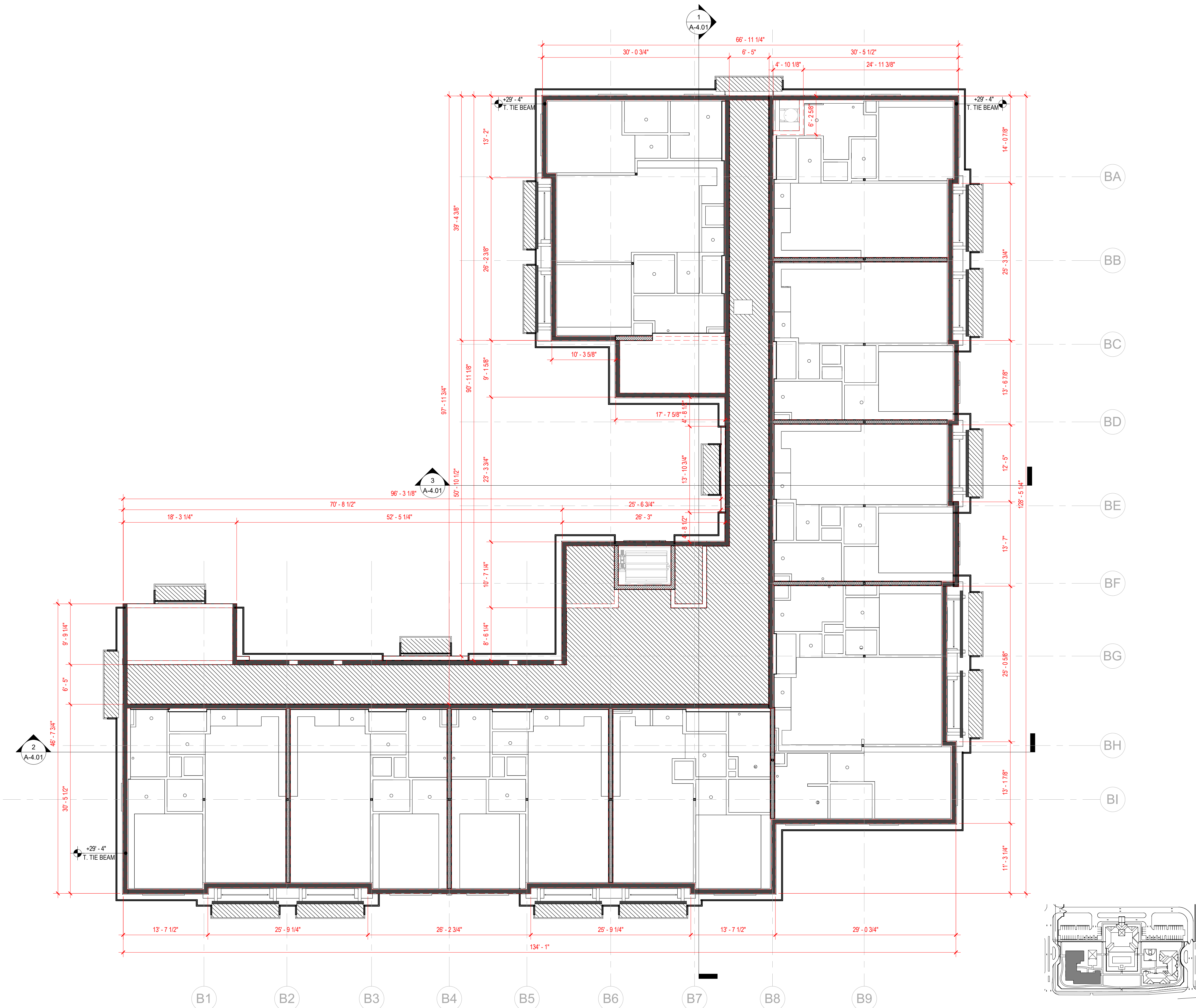
BUILDING A KEY PLAN
